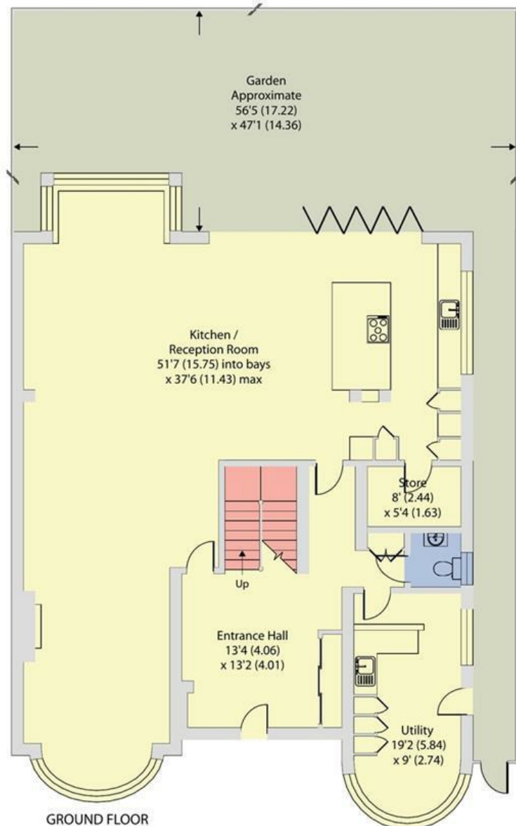
GROUND FLOOR
